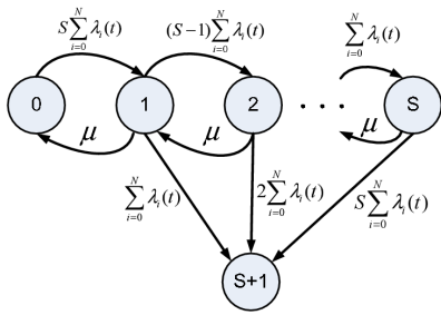
Fig. 2: State transition of the non-homogeneous CTMC. of reliability over the lifespan of the SSD array. The CTMC is non-homogeneous , because the error arrival rate \lambda_i(t) is time-varying depending on the system age. Next, we show how to analyze this non-homogeneous CTMC.
