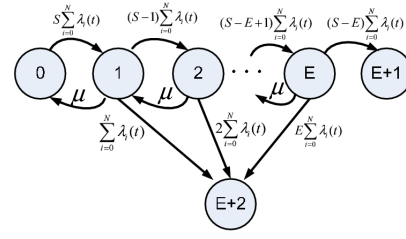
Fig. 3: State transition after truncation.
